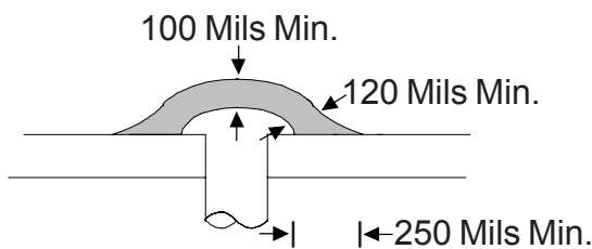
RIVET MANUFACTURED HEAD OR RIVET UPSET HEAD
